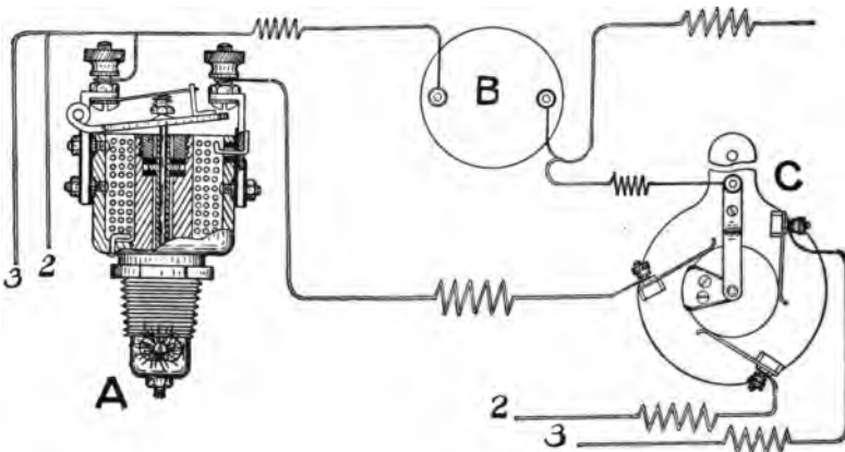
FIG. 200.—Three-Cylinder Circuit Diagram of the Durvea Exploder. A, exploder plug showing interior; B, retardation coil; C, contact breaker; 2 and 3, leads to second and third cylinder exploder plugs.
